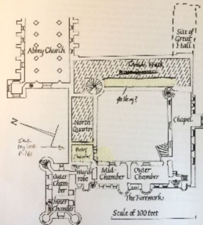
Fig. 1. Sketch plan of part of the Palace of Holyroodhouse in the mid 15th century
