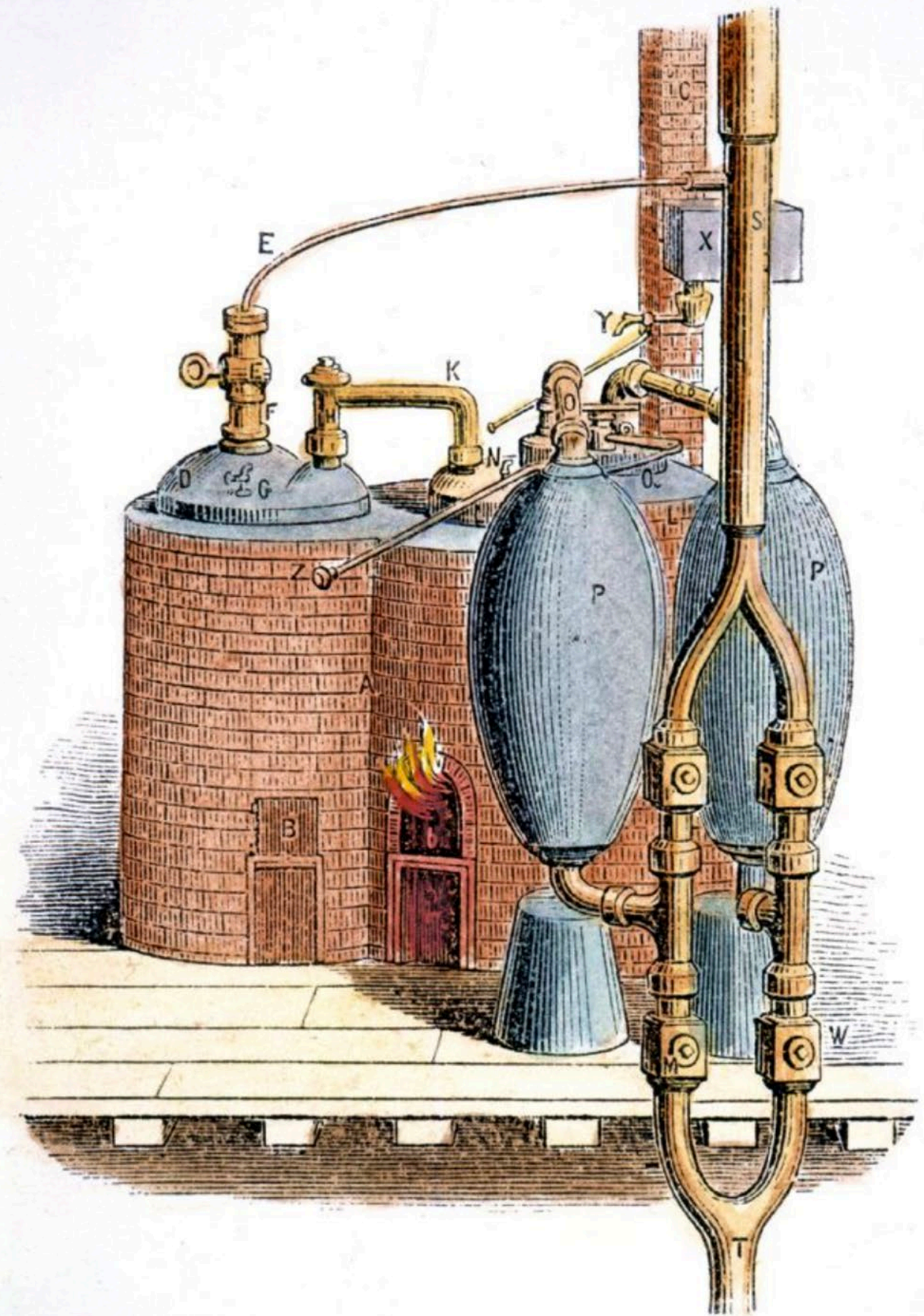
FIG. 8.—SAVERY'S ENGINE, A. D. 1699.
